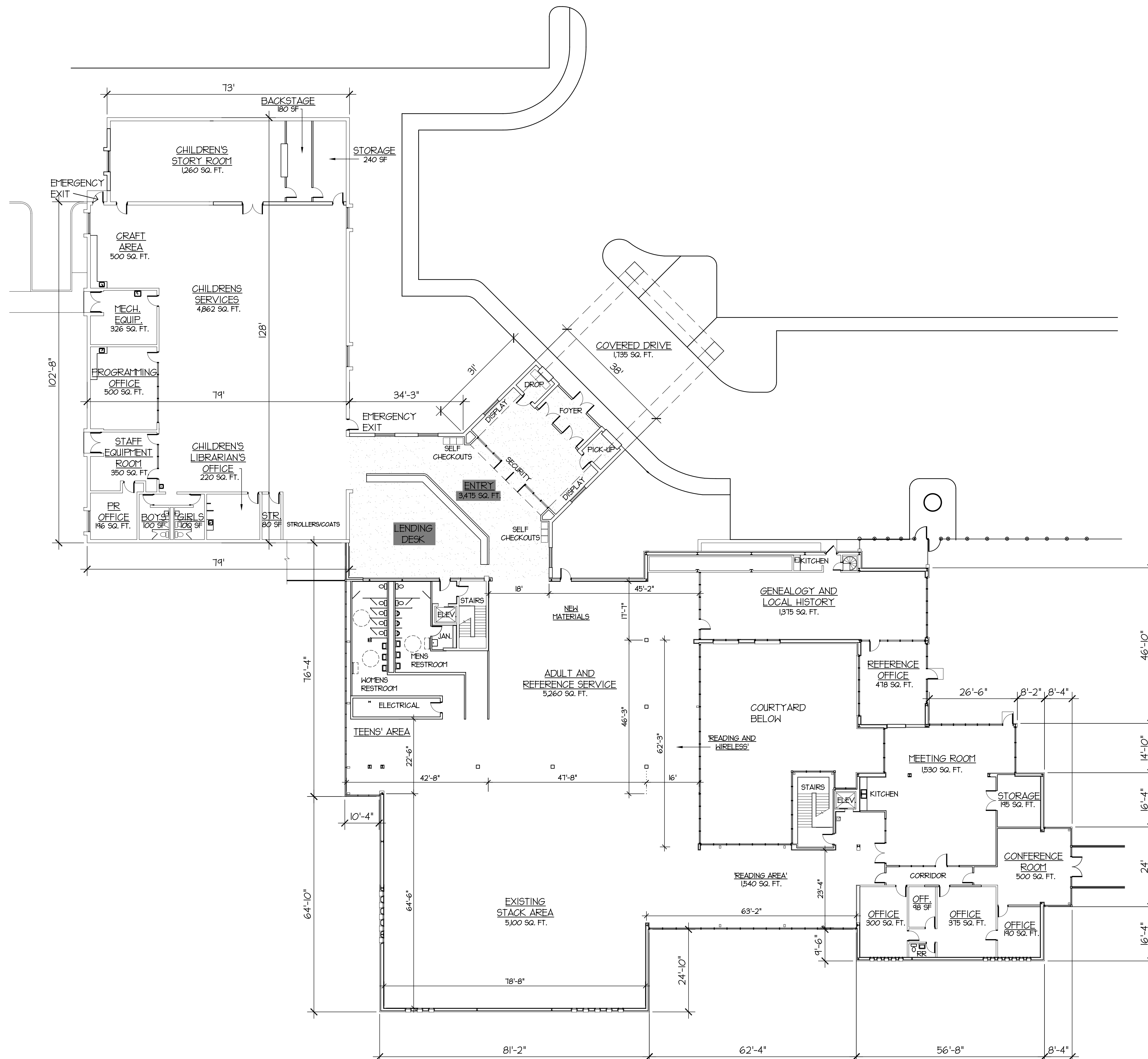
1 A-1 UPPER LEVEL FLOOR PLAN - PROPOSED SCALE: 1/16" = 1'-0" ORIGINAL UPPER FLOOR PLAN = 23,600 SQ. FT. CHILDRENS WING FLOOR PLAN = 9,960 SQ. FT. NEW ENTRANCE W/ COVERED DRIVE = 5,210 SQ. FT.
